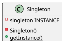
Figure 305: The UML diagram for a singleton pattern
